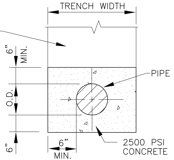
CONCRETE ENCASEMENT
