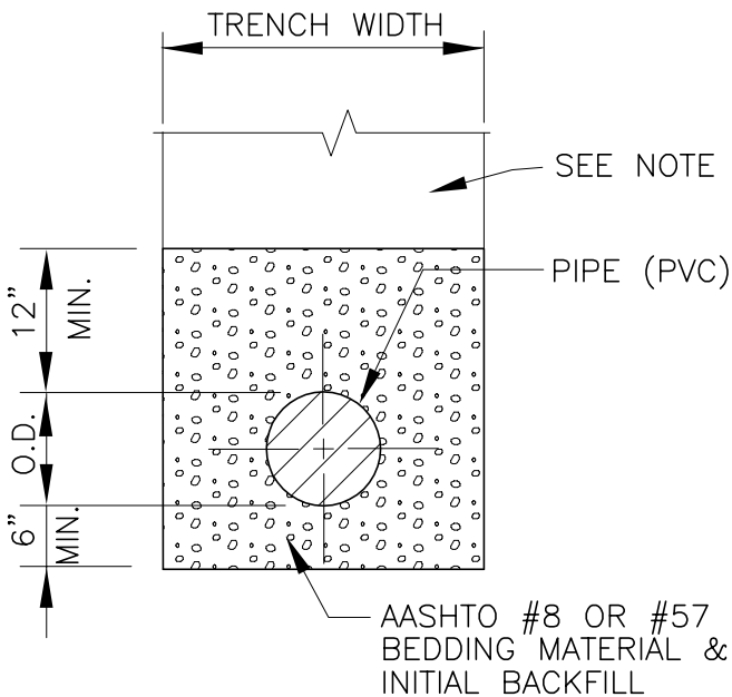
STANDARD BEDDING
